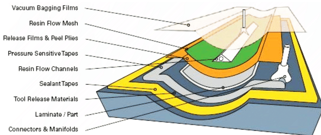
Fig.1 Principle of vacuum infusion
